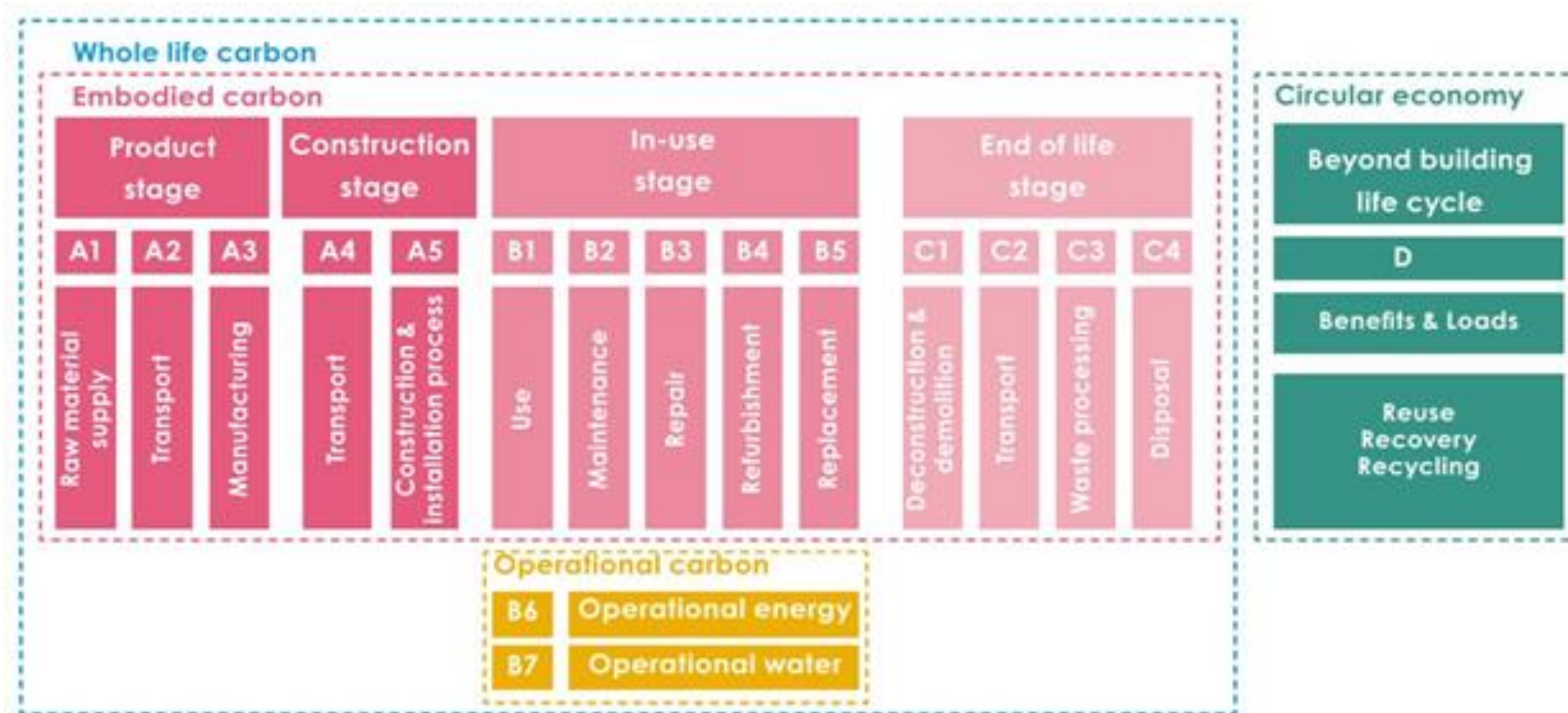
Figure 20.1: Diagram showing the stages of a lifecycle GHG emissions assessment. Diagram taken from the LETI (2020) Embodied Carbon Primer, based on lifecycle stages set out in BS EN 15978:2011 Sustainability of Construction Works – Assessment of Environmental Performance of Buildings – Calculation Method.
